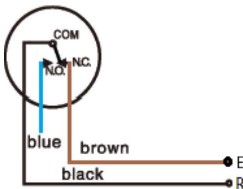
High Level Float wiring
